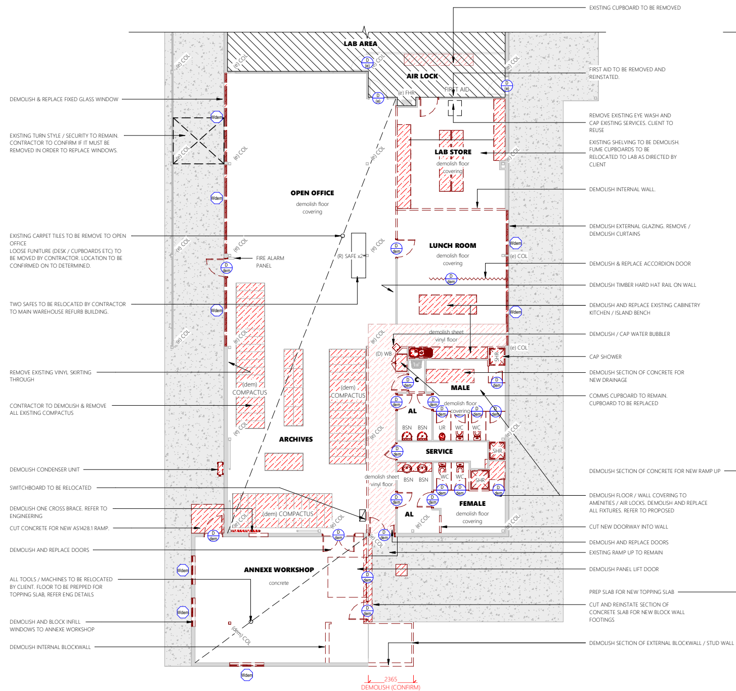
Existing Registry Floor Plan
