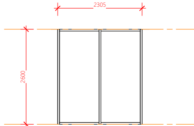
WINDOW TYPE C
