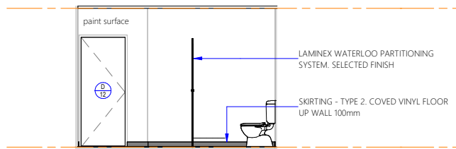
Elevation 4H
