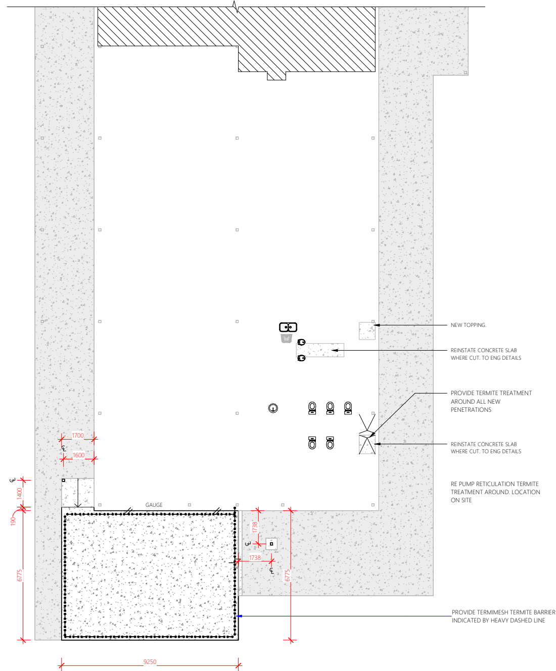
Proposed Slab Plan
