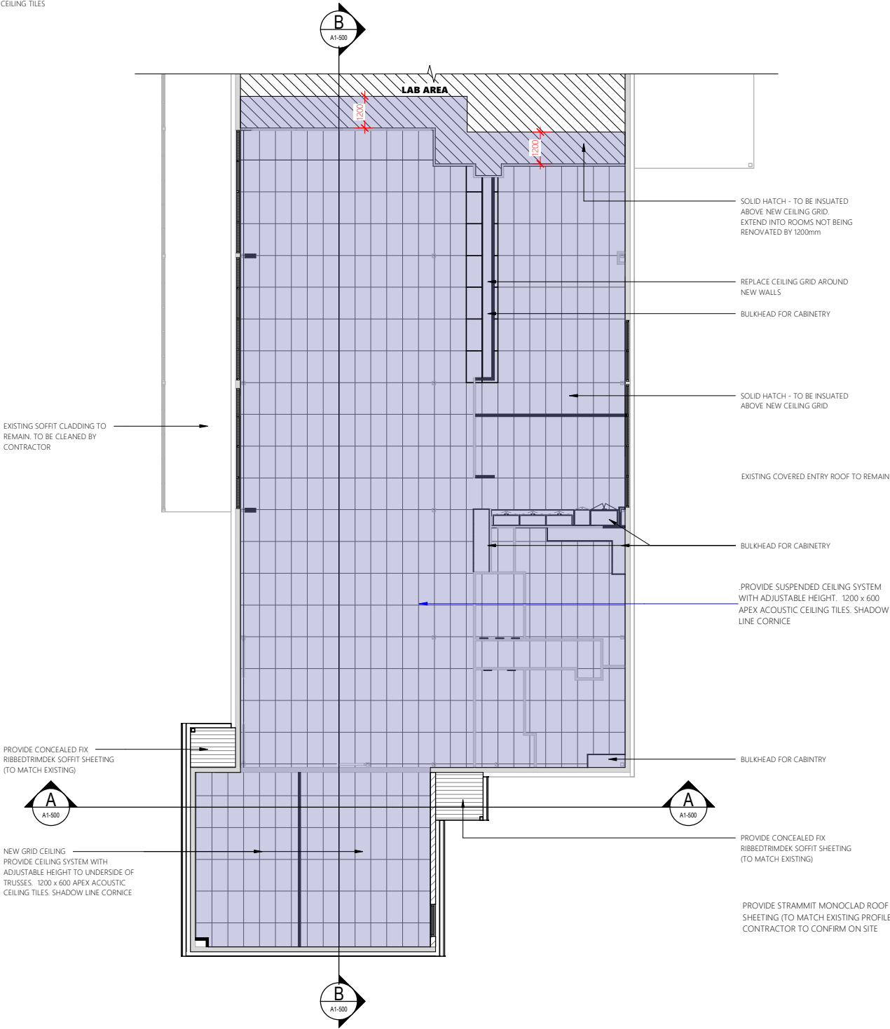
Proposed Ceiling Plan
