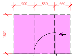
HINGE-SIDE APPROACH DOOR OPENS TOWARDS USER
