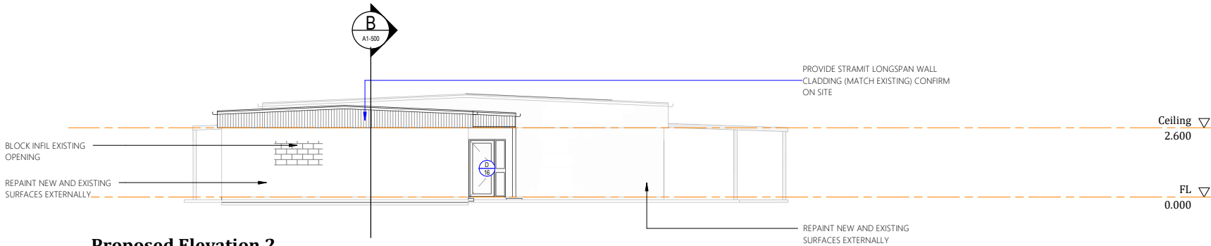
Proposed Elevation 2 1 : 100
