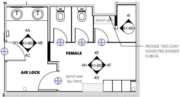
Internal Plan 4
