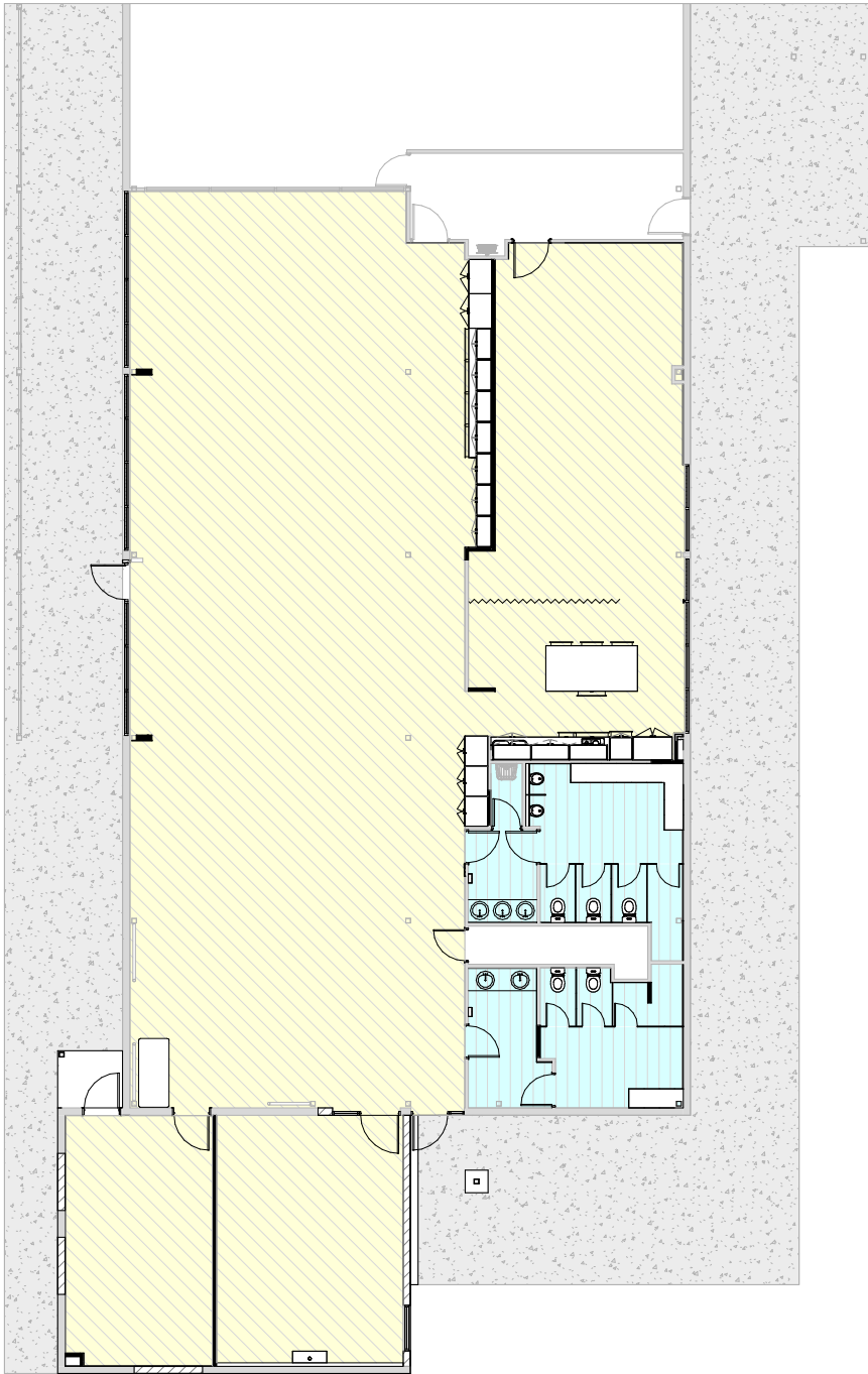
Floor Covering Plan
