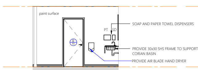
Elevation 4D
