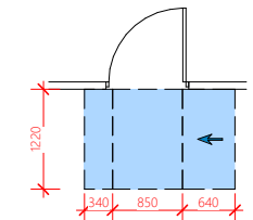
HINGE-SIDE APPROACH DOOR OPENS AWAY FROM USER
